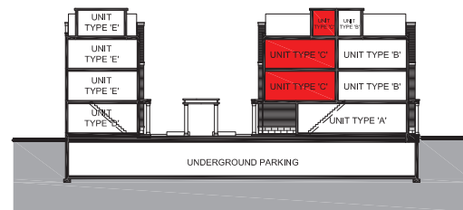
BUILDING SECTION
